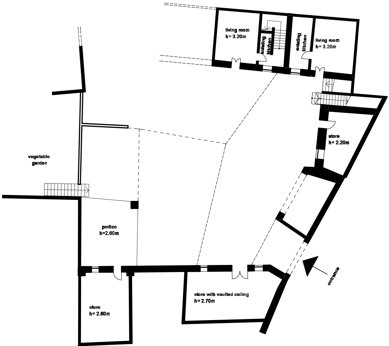
Existing Ground Floor Plan 1:200
